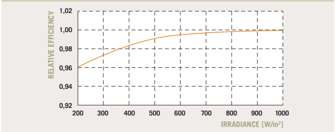
The typical relative change in module efficiency (at nominal power) at an irradiance of 200 W/m 2 in relation to 1000 W/m 2 (both at 25 °C and AM 1.5 spectrum) is -4.0 % rel.
